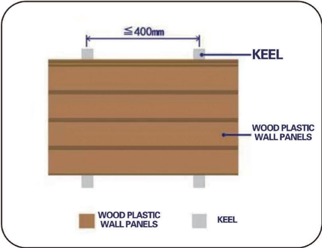
INSTALLATION DIAGRAM OF WOOD PLASTIC WALL PANELS
